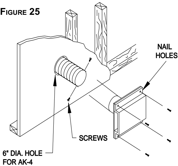
COMBUSTION AIR ASSEMBLY FOR MODEL NO. AK-4
